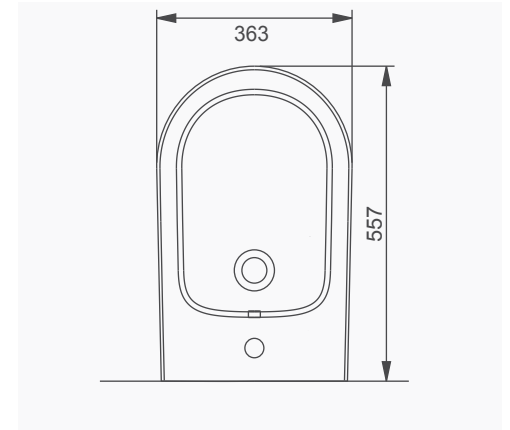
A011112 WC PAN WITHOUT BIDET FUNCTION
