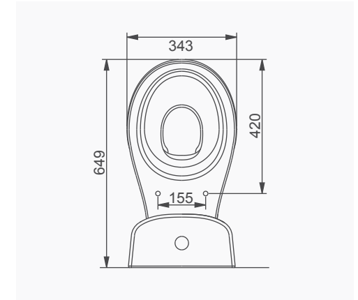
A051011 WC PAN WITHOUT BIDET FUNCTION
