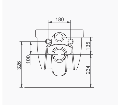
TERRA RIM-OUT ASMA KLOZET /TERRA RIM-OUT WALL-HUNG WC PAN A011111 KLOZET / WC PAN A010001 YAVAŞ KAPANIR KAPAK /SEAT & COVER SOFT CLOSE
