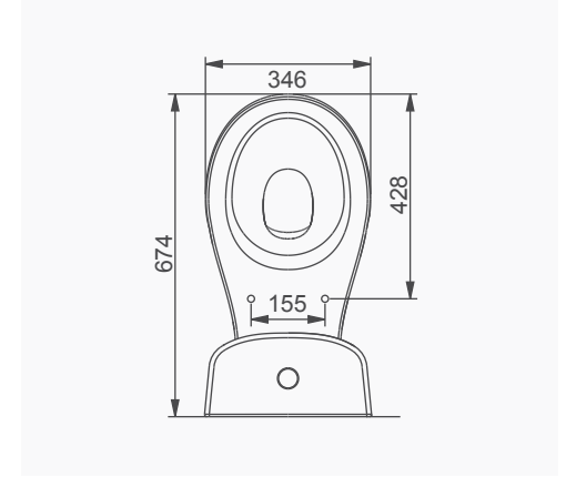
A051012 WC PAN WITHOUT BIDET FUNCTION
