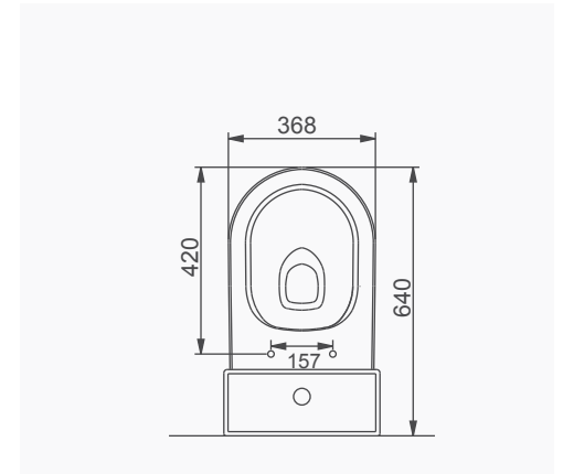
A031002 WC PAN WITHOUT BIDET FUNCTION
